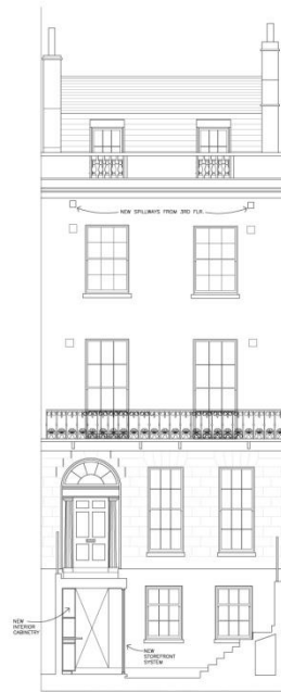
① FRONT ELEVATION 1M 2M
