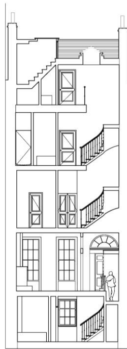
section CC
